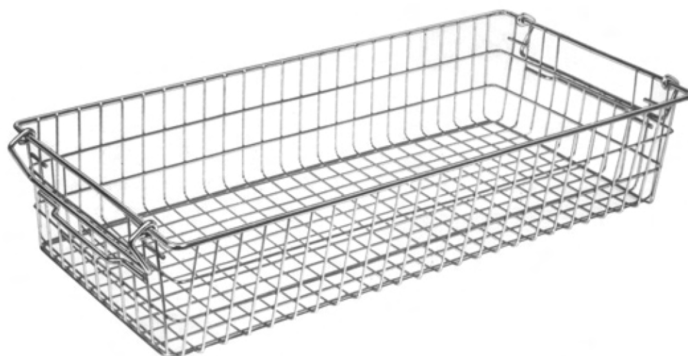
19-219 (60 x 30 x 15 cm) Nominal dimensions
