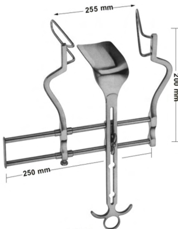
06-261 BALFOUR Lateral blades 105 mm deep Center blade 107x 59 mm
